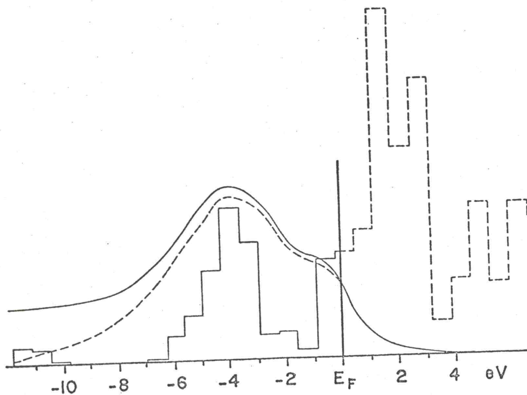
FIG. 15. Nb-L III emission from NbC.
