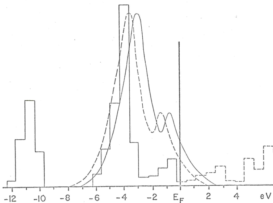
FIG. 16. Nb-M IV,V emission from NbC.
